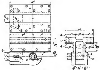
Figs. 1078-1080. Laird Crosshead. Baldwin Locomotive Works.
